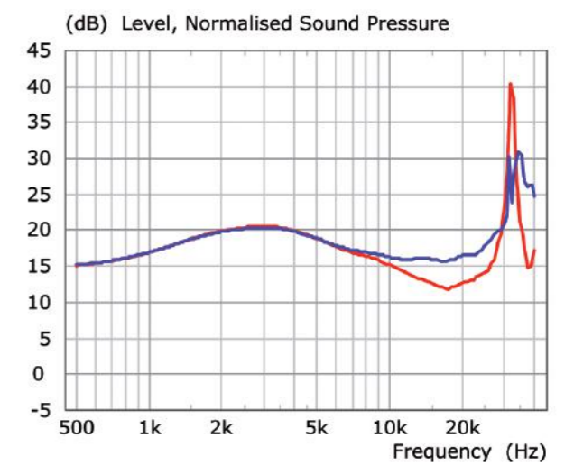
Figure 23 Simulated response of tweeter — without tangerine waveguide — with tangerine waveguide
