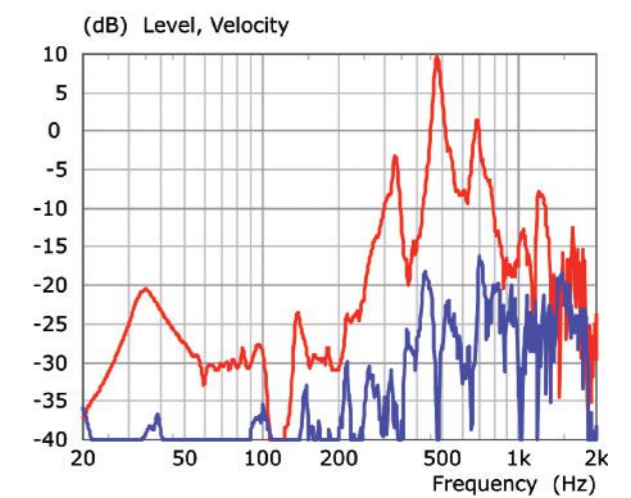
Figure 3 Panel vibration — without damping — with damped bracing
