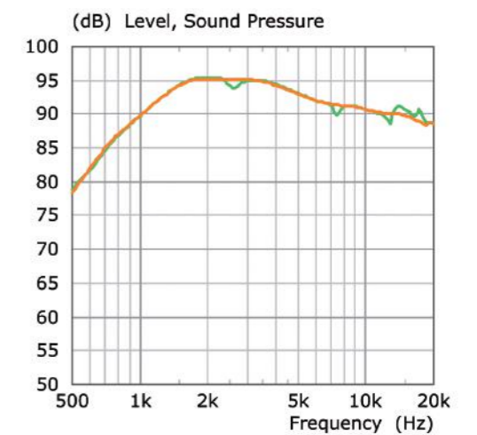
Figure 15 Simulation of tweeter response — In perfect waveguide — With open gap
