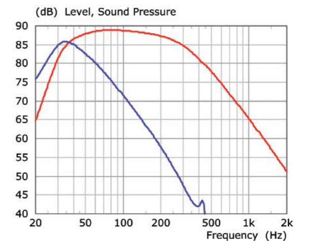
Figure 7 Simulation of bass driver + port — and port only —when the port is placed close to the antinode of internal resonances.
