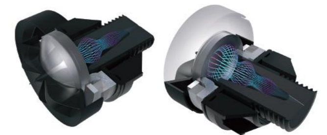
Figure 24 Front and rear view cross sections of tweeter showing rear loading
