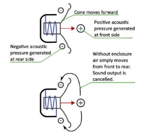
Figure 1 Driver in free air
