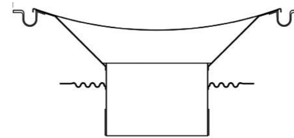
Figure 9 Cross-section of bass driver moving parts
