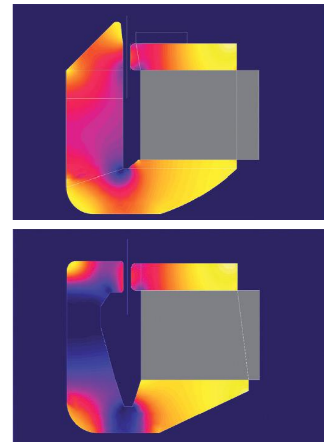
Figure 11 Finite Element Analysis (FEA) of Top – 2011 R Series bass driver magnet system Bottom – 2018 R Series bass driver magnet system
