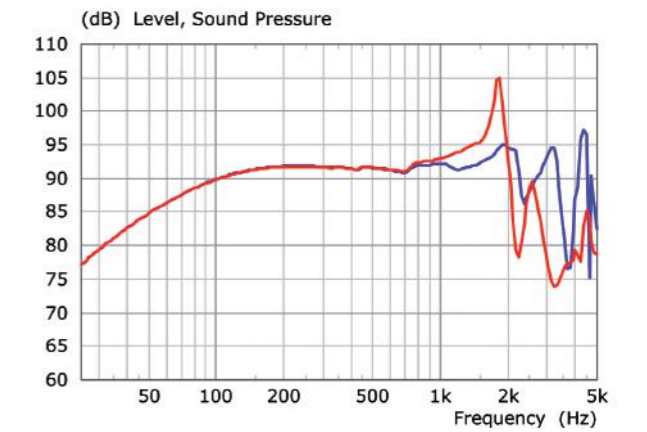
Figure 10 — Response of non-optimised bass driver — Response of optimised bass driver Panel
