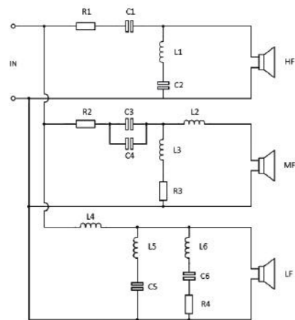
Figure 25 General schematic of R Series 3-way crossovers
