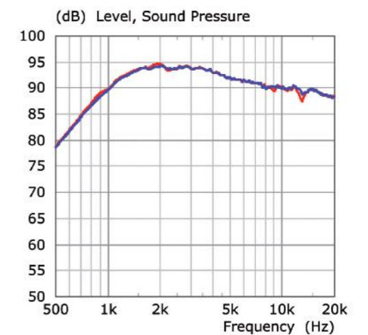
Figure 16 Actual tweeter response — Original — With cavity damping
