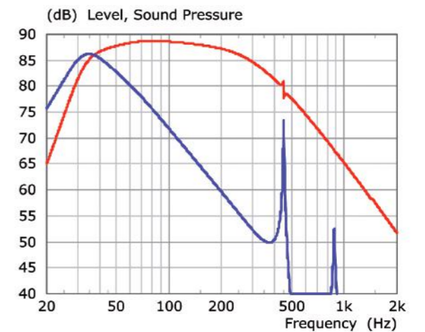
Figure 6 Simulation of bass driver + port — and port only —when the port is placed close to the node of internal resonances.
